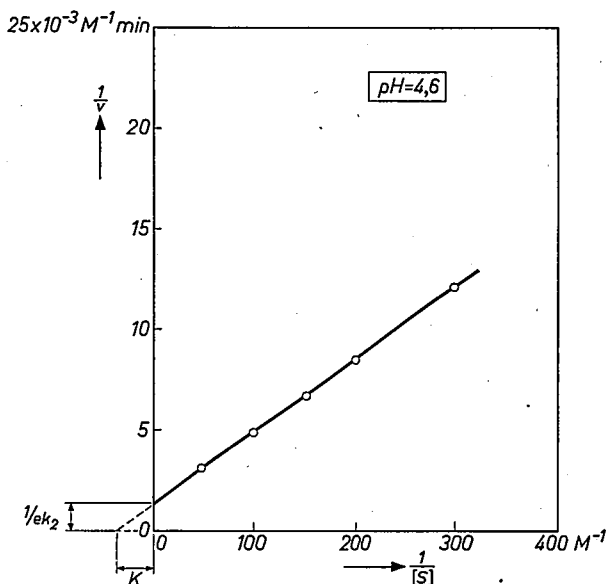
Fig. 4. Hydrolysis of benzoylarginine ethyl ester by the action of papain at pH = 4.6 . The reciprocal of the hydrolysis rate 1/v is plotted versus the reciprocal of the concentration 1/[S] of benzoylarginine ethyl ester.
