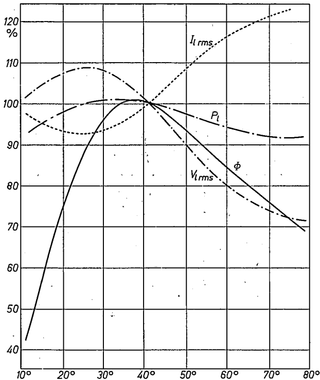
Fig. 13. Luminous flux \Phi , r.m.s. value of the lamp voltage v_{l\text{ r.m.s.}} , r.m.s. value of the lamp current i_{l\text{ r.m.s.}} and power P_l for a fluorescent lamp, as a function of the temperature of the glass wall. The lamp is connected to a constant-voltage mains supply by means of a ballast choke.
