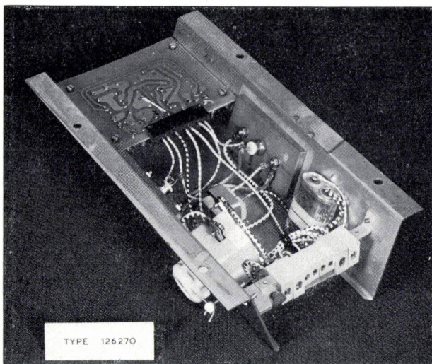
Fig. 10. A dimmer which uses the circuit of fig. 9, shown open. When closed, the dimensions are 21 \times 35 \times 8 cm.
