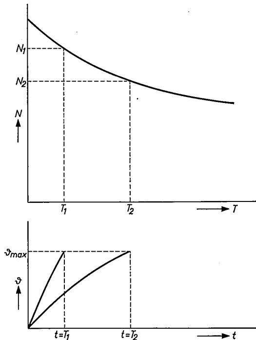
Fig. 4. Load characteristic of a diagnostic X-ray tube: the permissible (constant) load N is plotted against exposure time T . The lower graph shows the temperature \vartheta at the focus, for two loads N_1 and N_2 , as a function of time t . The maximum permissible temperature \vartheta_{max} is reached exactly at the end of the respective exposure times T_1 and T_2 .
