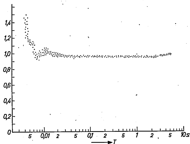
Fig. 22. Delivered dose for a large number of radiographs at different exposure times, made with the Amplitat controlling a six-peak generator. The dose actually delivered was measured with a dosimeter at the normal film location. The deviations from the nominal value (here put at 1) only exceed 20% for switching times below 5 ms.
