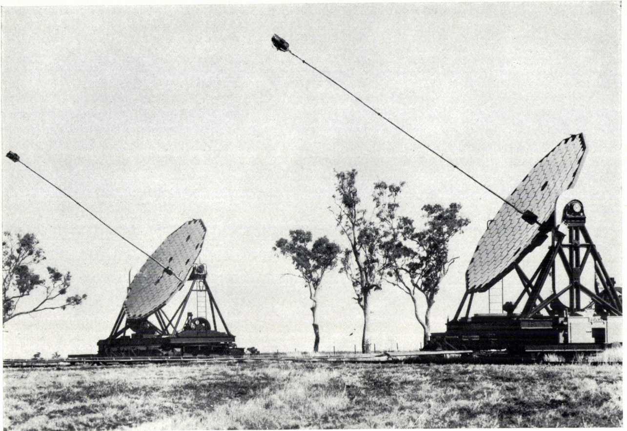
Fig. 8. The reflectors. Each reflector consists of 252 hexagonal mirrors and has a diameter of about 6.7 m. The pole carrying the photoelectric detector is 11 m long.
