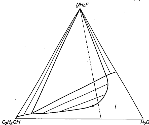
Fig. 23. Isothermal cross-section of the system \text{H}_2\text{O} - \text{C}_2\text{H}_5\text{OH} - \text{NH}_4\text{F} at 25 °C (concentrations in weight percentages). Following the dashed line upwards we see that \text{NH}_4\text{F} is initially simply soluble in a water-alcohol mixture, but at a certain concentration there is a separation into a high-water and a high-alcohol phase. This is the basis of the familiar method of separation by salting-out ; the salt \text{NH}_4\text{F} expels the alcohol from the water-alcohol mixture.
