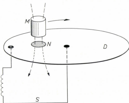
Fig. 8. Diagram of the superconducting dynamo. The permanent magnet M induces a normal, non-superconducting region N in the superconducting disc D and some flux from M penetrates through N . When M rotates around the centre of D so that N passes repeatedly through the terminals of the superconducting circuit S , flux is pumped into S and the persistent current is changed.
