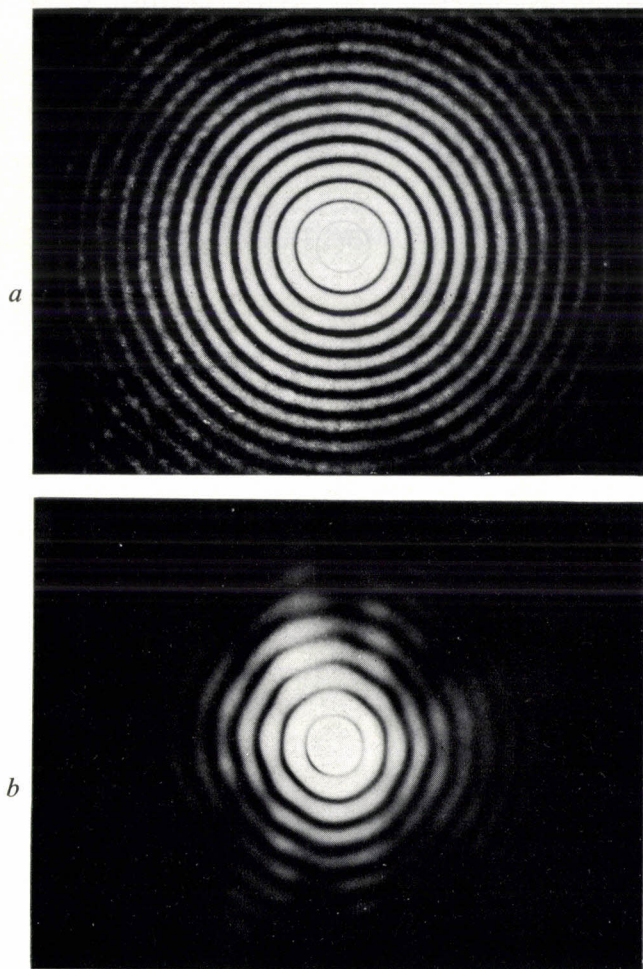
Fig. 4. Diffraction patterns for die bores. a ) Bore of diameter 136 \mu\text{m} , reasonably circular. b ) Bore of diameter 50 \mu\text{m} , somewhat octagonal. (The magnification of photographs ( a ) and ( b ) is not identical.)
