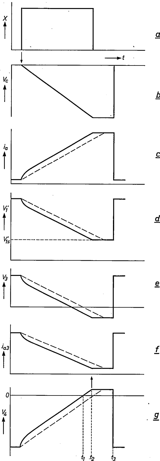
Fig. 19. Waveforms of the various signals. The X-radiation in this case is assumed to be constant. At t_1 the thyatron ignites, at t_2 the relay S_1 releases and at t_3 the relay S_8 releases.
