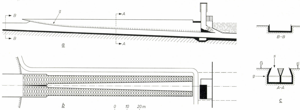
Fig. 15. Entrance area of the Coen tunnel under the North Sea Canal (after Griffioen [15]). a) Longitudinal section. b) Plan view. c) Two transverse cross-sections. A grid g is fitted at approximately constant height above the road surface. The grid receives its light by way of a gradually narrowing opening s .
