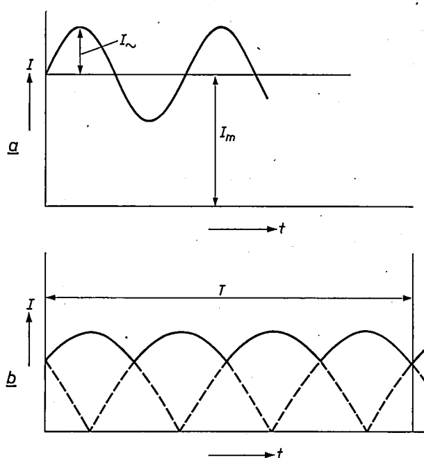
Fig. 17. Examples of a d.c. current with superimposed ripple. a) Sinusoidally modulated d.c. current. I_m average current. I_{\sim} amplitude of sine wave. b) Rectified alternating current consisting of four sine pulses ( p = 4 ).
