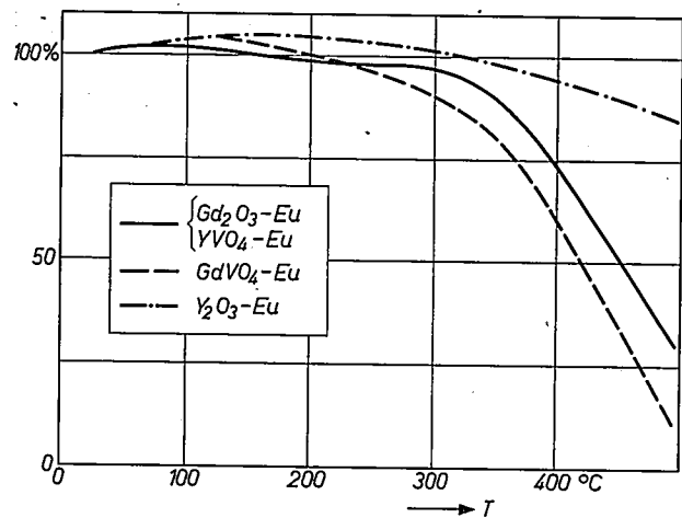
Fig. 6. Intensity of the fluorescent radiation of some Eu phosphors plotted against temperature. The intensity at room temperature is assumed to be 100%. Up to 300 °C the temperature has hardly any effect.
