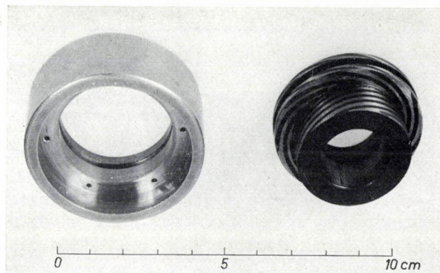
Fig. 2. Parts of the new spiral groove bearing. The cylindrical bearing housing is shown on the left, and the rotating part, made of hard material that is attached to the straight-through shaft is shown on the right. Here the groove patterns (1, 2, 4 and 5 in fig. 1) are not cut in the wall of the bearing housing, but in the hardened moving part; this makes no difference to the operation of the bearing. The moving part is shown the opposite way round from the housing so that the groove patterns may be seen. The ends of the grease channels, which, in this design, run in a slightly different way from that shown in fig. 1c (7), may be seen in the bearing housing.
