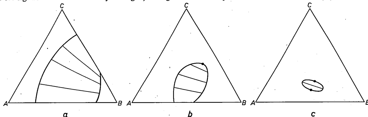
Fig. 7. Three isothermal cross-sections of the same system, obtained at successively higher temperatures. a ) Miscibility gap in the form of a strip. b ) Miscibility gap at a boundary. Unlike the type of miscibility gap in fig. 6 , the mutual miscibility of A and B decreases when a small amount of C is added. c ) Closed miscibility gap, with two critical points.
