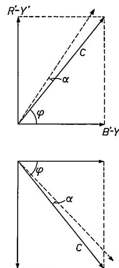
Fig. 15. Vector diagram of the chrominance signal of PAL for two successive lines, where there is a differential phase error \alpha . The vectors shown in broken lines occur instead of the solidly-drawn vectors C . Because \varphi changes its sign each time, while \alpha does not, there is a certain amount of phase error compensation in PAL.
