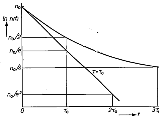
Fig. 2. Variation with the time t of the concentration n of the electrons in the conduction band after the illumination is switched off. If the recombination is a monomolecular process, n decreases exponentially and with log-linear co-ordinates the curve is a straight line of negative slope. With bimolecular recombination a curve is found whose slope with increasing t becomes steadily less steep. The curves apply to cases where the initial concentrations n_0 and the initial slopes are equal (cf. II,7 and II,8).
