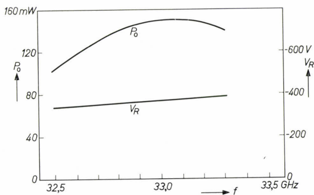
Fig. 5. Variation of the output power P_o with frequency f for tuning by the method in fig. 3b, from measurements on a random sample. V_R corresponding reflector voltage.
