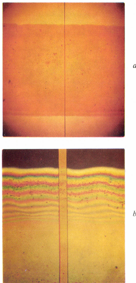
Fig. 10. a ) Photo-micrograph of thin-film transistor of the type in fig. 2 d with channel of CdSe. The thin vertical line is the gate electrode. The two other electrodes and the channel cannot be separately distinguished; they form together the dark horizontal strip. b ) Detail of the edge of the channel adjoining the gate (i.e. the vertical golden strip) looked at through the substrate. The coloured wavy lines are interference fringes in the thin region at the edge of the channel (magnification 475 \times ).
