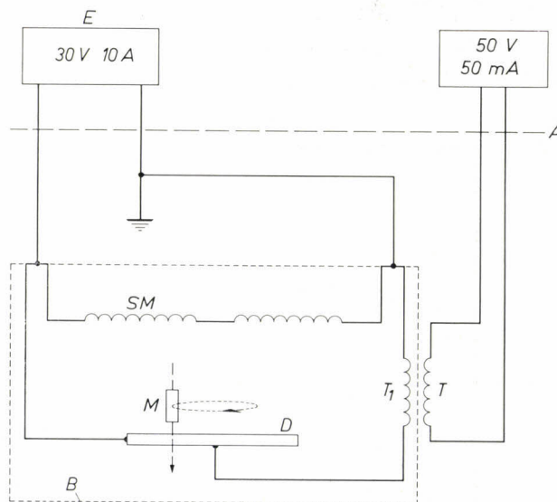
Fig. 7. Magnet current supply diagram. The persistent current in the superconducting circuit (within the contour B) is established by: a) activating the "thermal switch" TT_1 (i.e. disturbing the superconduction in the coil T_1 by a small current through T heating T and T_1 ); b) connecting the external supply E and setting the current; c) de-energizing the thermal switch TT_1 . As soon as T_1 is superconducting again, a persistent current flows in B and E can be disconnected. SM superconducting coils. M, D superconducting dynamo. The parts drawn above line A are outside the cryostat.
