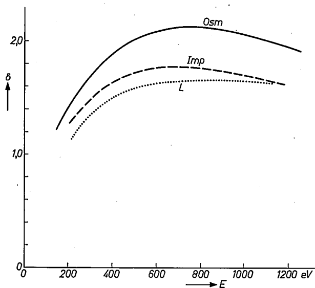
Fig. 7. Secondary emission coefficient \delta as a function of the energy E of the primary electrons (in eV) for a normal L cathode (L), an impregnated cathode (Imp) and an osmium-coated L cathode (Osm).
