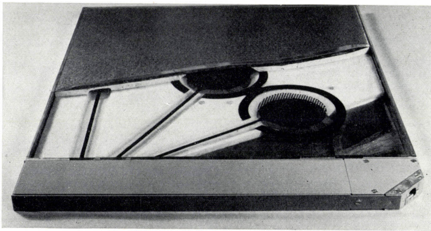
Fig. 11. Ionization chamber, partly cut open, showing the electrode systems for two of the measurement fields.
