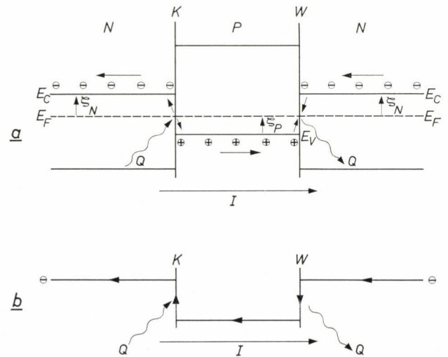
Fig. 7. a) The energy bands in a combination of an N -type and a P -type semiconductor. E_F Fermi level. E_C lower edge of conduction band in the N -type semiconductor. E_V upper edge of the valence band in the P -type semiconductor. I electric current. At the cold junction K hole-electron pairs are generated, and thermal energy Q is taken up. At the hot junction W an amount of heat Q is given up upon recombination. \zeta_N = E_C - E_F , \zeta_P = E_F - E_V . b) The energies of the conduction states in a circuit of two semiconductors. At the cold junction K the conduction electrons are excited to a higher energy state by thermal energy taken up from the environment. At the hot junction W they return to the lower state, and heat Q is given up.
