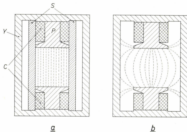
Fig. 5. a) Cross-section of the superconducting magnet. Y yoke and P pole pieces of mild steel. C superconducting coils of niobium-zirconium wire. S superconducting shields of lead-bismuth. The lines of magnetic field are shown dashed. b) To show the effect of the shields S, the field pattern that would be obtained without the shields is shown.
