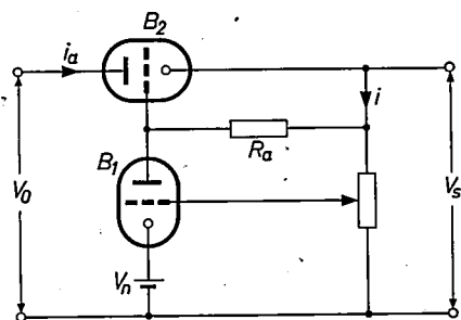
Fig. 14. Circuit showing the principle of a stabilized power supply.
