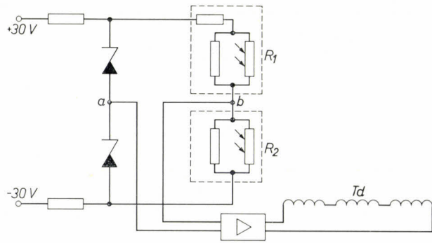
Fig. 14. Circuit for automatic control of the light level in a road tunnel as a function of the luminous intensity outside the tunnel. A number of light-sensitive resistors are incorporated in each of the resistor combinations R_1 and R_2 . (Only one of these has been drawn.) R_1 and R_2 are placed outside and inside the tunnel, respectively. T_d indicates the control windings of the three saturable reactors of a central control box (see fig. 11).
