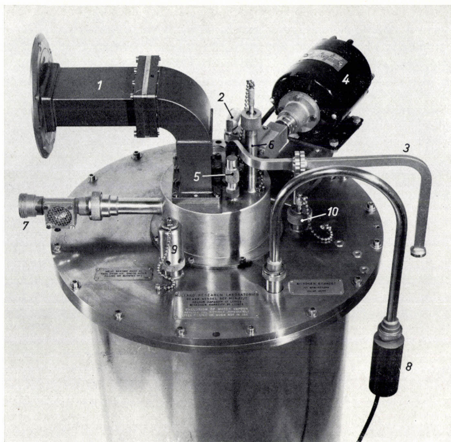
Fig. 12. The top of the cryostat. 1 input waveguide. 2 coaxial output. 3 pump waveguide. 4 motor for driving the superconducting dynamo. 5 magnetic field orientation adjustment. 6 helium filling tube. 7 helium exhaust. 8 electrically heated "bunsen valve" preventing water from entering the nitrogen dewar. 9 nitrogen safety valve. 10 nitrogen filling tube.
