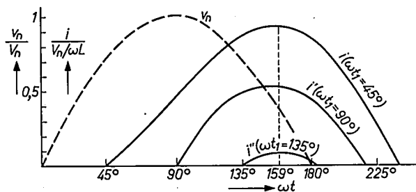
Fig. 3. Curves for a half-cycle of the mains voltage v_n and of the current in the circuit shown in fig. 2. The three current curves i , i' and i'' apply to the cases where the control signal is applied to the thyristor at the instants of time given by \omega t_1 = 45^\circ , \omega t_1 = 90^\circ and \omega t_1 = 135^\circ . The ratio between the maintaining voltage of the lamp V_1 and the r.m.s. value of the mains voltage has been taken as 0.35.
