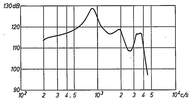
Fig. 12. The maximum output signal of the KL 6710/01 hearing aid as a function of frequency using elbow No. 2 and with the tone control at "normal". The input signal is raised until there is no further alteration in the output signal, shown by the curve in dB with respect to the reference level of 2 \times 10^{-4} \mu bar.
