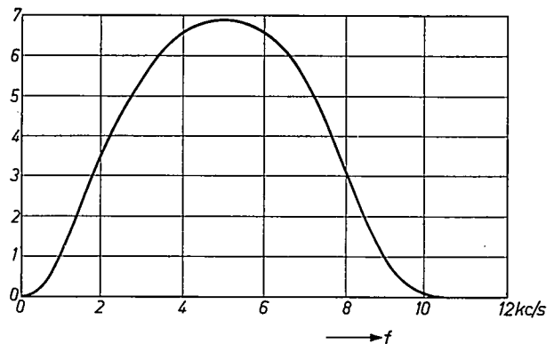
Fig. 1. Frequency characteristic of a "psophometric filter", as used in noise measurements to represent the differences in the subjective effect of audible interfering sounds having the same energy level but different frequencies.
