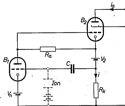
Fig. 15. Circuit of the pre-amplifier incorporated with the ionization chamber. B_1 special electrometer valve with grid current < 10^{-12} A and indirectly heated cathode (used for mechanical stability). The quiescent current i is kept constant by means of the reference-voltage source V_n . The quantity to be measured is the change in i_a that occurs as soon as the ionization chamber I_{ion} supplies a charging current to the capacitor C . This change is proportional to the dose reached.
