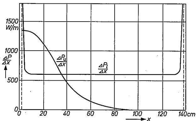
Fig. 8. Distributions of effective power P_u and the power loss P_1 which are required to give the furnace discussed in this article a uniform temperature.
