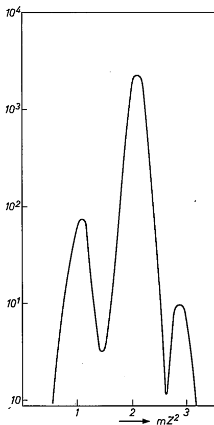
Fig. 12. Spectrum of mZ^2 values ( m = nuclear mass and Z = atomic number) obtained in measurements made with a particle-identification system on a beam containing protons, deuterons and tritons; we have taken mZ^2 = 1 for the proton. The value of mZ^2 is calculated for each incident particle from the product of the particle energy E and the energy loss per unit path length dE/dx . These two quantities are measured with separate detectors.
