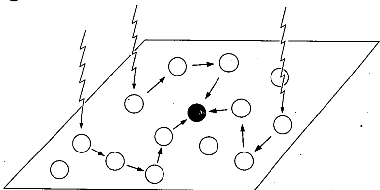
Fig. 11. Diagrammatic representation of the primary transfer of energy in photosynthesis. Excited chlorophyll molecules pass the excitation energy on to neighbouring molecules. One in about three hundred chlorophyll molecules, the "reaction centre", is able, very likely on account of its special bonding to donor and acceptor molecules, to utilize the excitation energy for an oxidation-reduction reaction.
