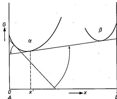
Fig. 2. Part of a G-x diagram of a binary system with phases \alpha and \beta . If a tangent is rolled around the G-x curve of the \alpha phase until it becomes tangent to the G-x curve of the \beta phase, the concentration range is found (from x = 0 to x = x' ) at which the phase \alpha is stable with respect to heterogeneous mixtures of \alpha and \beta .
