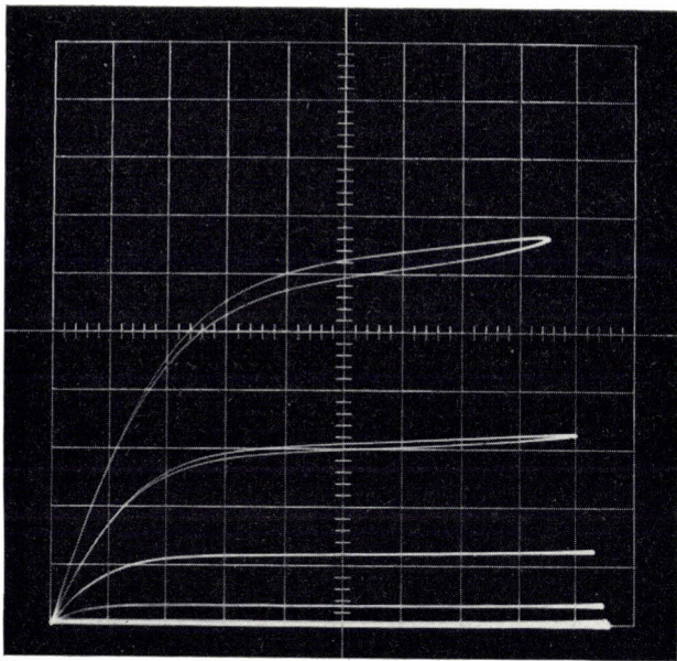
Fig. 6. The I - V_d characteristics of one of our thin-film transistors of the type illustrated in fig. 2d. One division on the I axis corresponds to 2 mA, and one division on the V_d axis corresponds to 1 V. The curves (from top to bottom) relate to V_g = 6 V, 5 V, 4 V, 3 V and 2 V respectively.
