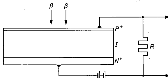
Fig. 11. In detectors for energy measurement on \gamma -quanta or long-range particles (high-energy \beta -particles) a P - N junction is not sufficient; such detectors should have a P - I - N configuration.
