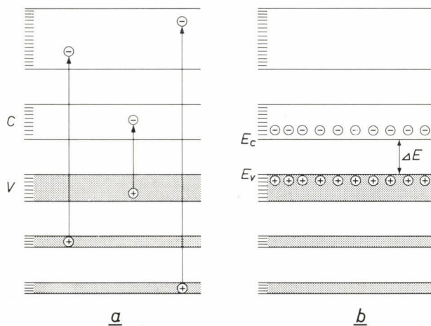
Fig. 5. a) Immediately after the incidence of a quantum or particle, there are free charge carriers in the conduction and valence bands ( C and V ) as well as electrons in higher bands and holes in lower bands.
