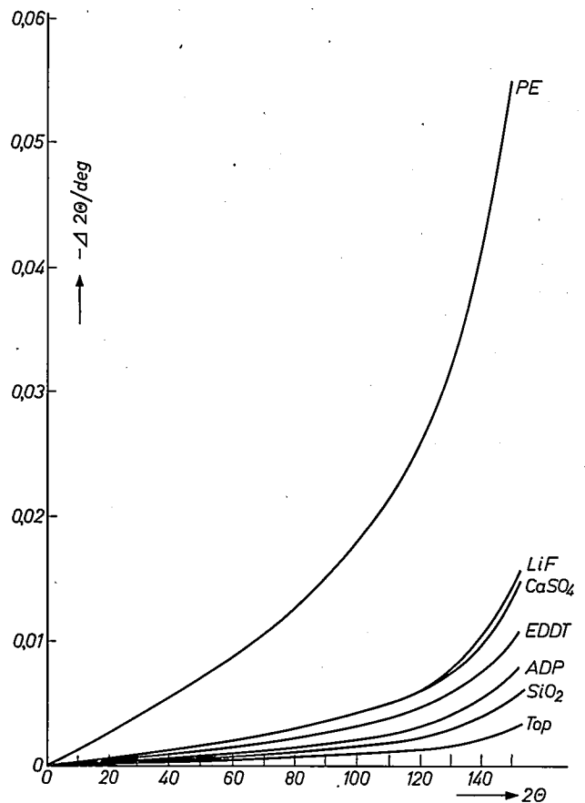
Fig. 7. Spectral line shift \Delta 2\theta for a 1^\circ change in the temperature of the analysing crystal, as a function of the total reflection angle 2\theta , for the seven crystals available in the spectrometer.
