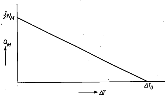
Fig. 11. Cooling power diagram after equation (19), giving the maximum cooling power Q_M as a function of the temperature reduction \Delta T . \Delta T_0 is the maximum temperature reduction. N_M is the electrical power consumed at \Delta T = 0 .
