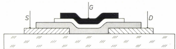
Fig. 8. Configuration of the type in fig. 2c, but now with the electrodes on either side of the channel.
