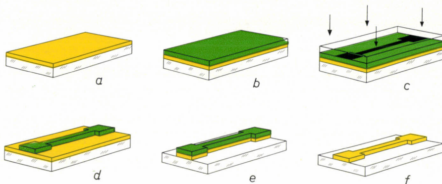
Fig. 5. The photo-etching method. a ) Substrate with metal layer (yellow); b ) the metal layer covered with a lacquer layer (green); c ) the lacquer layer is exposed through a photographic mask; d ) the lacquer is photographically developed; e ) the uncovered metal is etched away; f ) the residual lacquer is removed.
