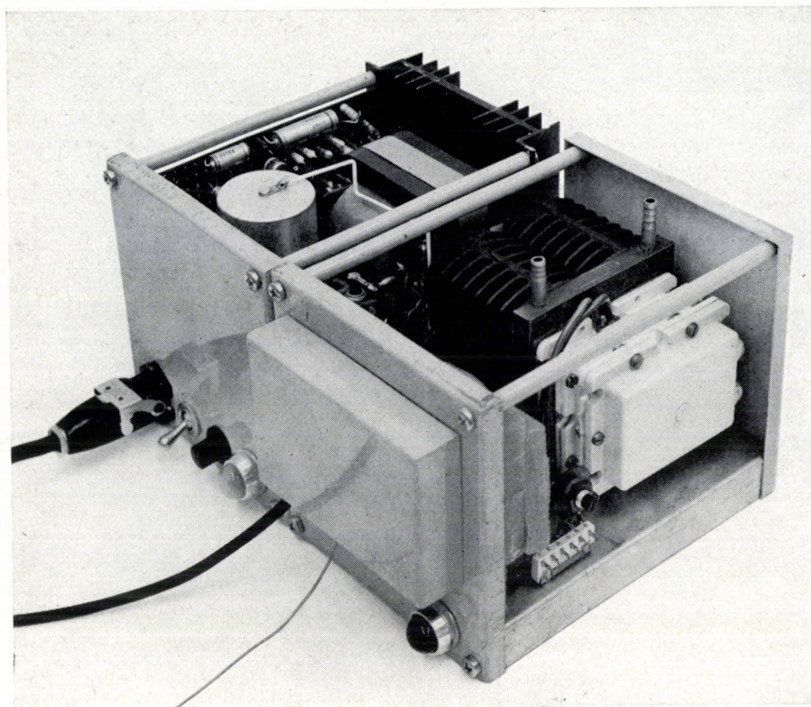
Fig. 22. Example of a freezing-point thermostat after Polnitzky [14]. The cover has been removed.
