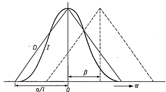
Fig. 8. Reflection coefficient I of a crystal as a function of the angle \alpha by which the angle of incidence deviates from that at which optimum reflection occurs. The triangle D represents the transmission of a collimator as a function of the angle between the direction of the collimator plates and that of the radiation. a is the spacing and l the length of the plates. The product of I and D determines the line profile measured. If the crystal is rotated through an angle \beta , the triangle D is displaced with respect to the curve I (dotted curve).
