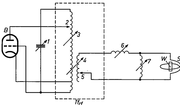
Fig. 2. Theoretical diagram of a generator for r.f. induction heating showing a few of the methods of adjusting the power. B is the oscillator tube, Tf the r.f. transformer, S the work coil and W the work-piece.
