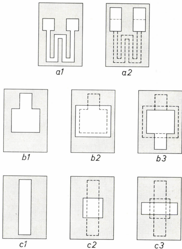
Fig. 4. The formation of a pattern by means of masks during evaporation. The masks that have to be used successively to form a given element are shown for three different elements.
