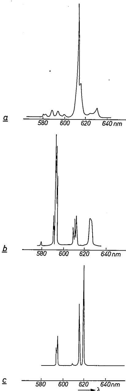
Fig. 5. The wavelengths of the lines of the fluorescence spectrum are hardly influenced by the nature of the matrix activated by europium. The spectra shown here are those of a ) Gd_2O_3-Eu , b ) Gd_2O_3.B_2O_3-Eu and c ) GdVO_4-Eu . In all three phosphors a cluster of lines is found between 590 and 600 nm and one between 610 and 620 nm. The intensity distribution, however, differs substantially. (The ordinate scales have been chosen so that the highest peaks in the three figures have about the same height.)
