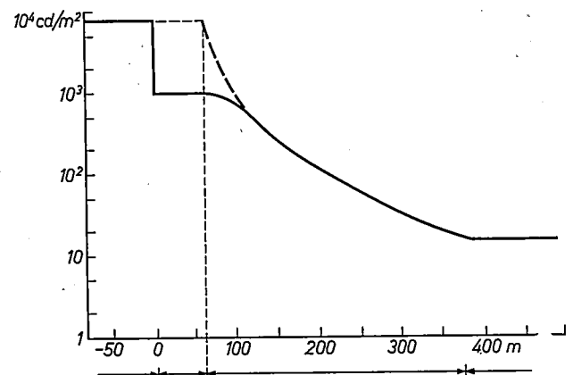
Fig. 14. Luminance transition necessary at the entrance of a tunnel so that a driver travelling at 72 km/h does not experience the black-hole effect or after-images.
