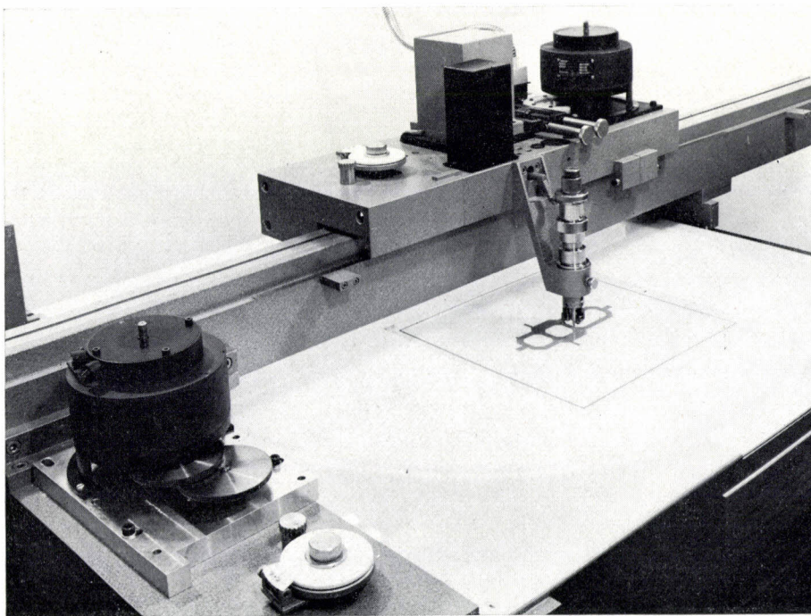
Fig. 8. An automatic drawing table used as an engraving machine. The upper support can be moved in the x -direction on a guide fixed to a second support, which can be moved along the y -direction (cf. fig. 7). The servomotors that can be seen in the photograph are used for the movement of the supports.
