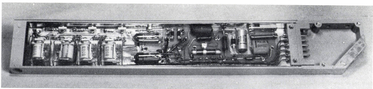
Fig. 17. The pre-amplifier opened up. It is located in the lower part of the ionization chamber casing shown in fig. 11 .
