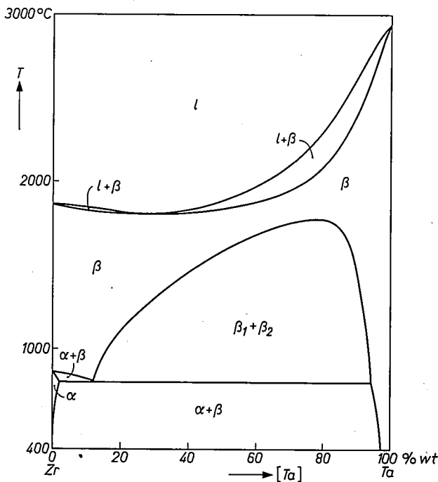
Fig. 16. Phase-diagram of the system Zr-Ta.
