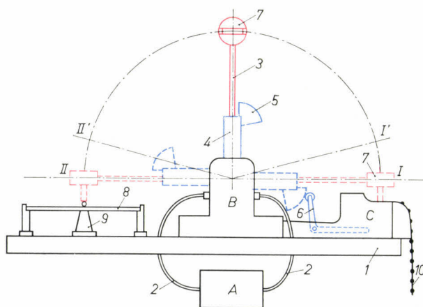
Fig. 2. Sketch of the mechanism of an arm unit. 1 is the bench top, and beneath it is located the driving mechanism A which, by means of Bowden cables 2, imparts a swinging movement to the arm 3 with its inserting head 7 (red). The mechanism B ensures that during its 180^\circ swing from "grip position" I to "insert position" II the arm also rotates 180^\circ around its own axis. The cam 5, fixed to the arm-holder 4, operates, through the lever 6 (blue), the mechanism C , which controls the feed of the component-strip 10. On coming down in position I the head cuts the connection wires of the component, bends them over and grips the component. In position II the connection wires are punched into the holes in panel 8 so that they bend over against the stops 9 and are thus fixed firmly to the panel.
