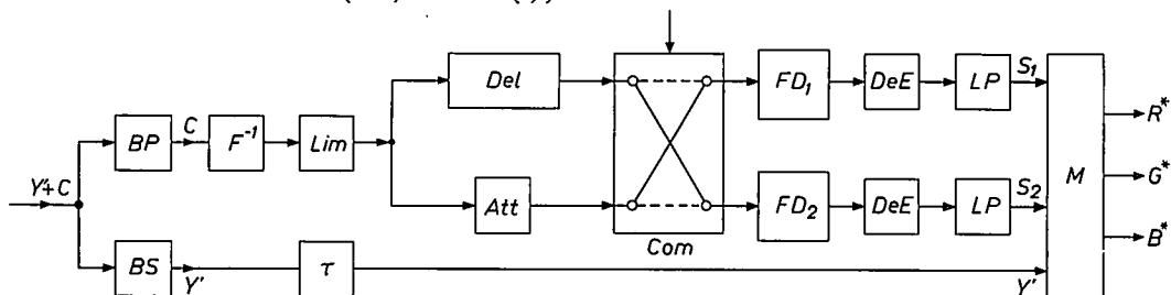
Fig. 14. Block diagram of a decoder for SECAM. The filters BP and BS separate the chrominance and luminance signals. The filter F^{-1} ("reshaping") cancels out the shaping provided at the transmitter. The amplitude of the signal is then limited (in Lim ), which helps to suppress noise. The signal then travels, through a delay line Del with a delay of one line interval ( 64 \mu s ) and an equivalent attenuator Att to the double changeover switch Com , which is switched over after every line scan and is so synchronized that the frequency discriminator FD_1 always provides the ( R' - Y' ) signal and FD_2 the ( B' - Y' ) signal. After compensation of the pre-emphasis, performed at the transmitter, in the de-emphasis stages DeE and band-limiting by means of the low pass the signals obtained are filters LP combined in matrix M with Y' to give the signals R^* , G^* and B^* .
