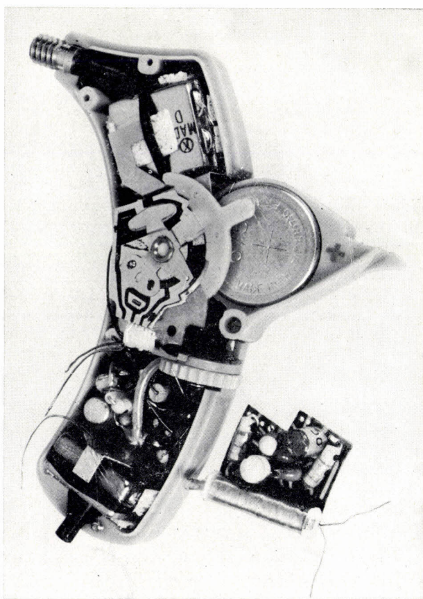
Fig. 8. The interior of the KL 6710/01 hearing aid.
