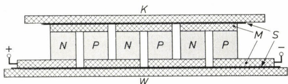
Fig. 4. Diagram illustrating the construction of a Peltier battery from a series of blocks of N -type and P -type semiconductors. M metal junctions. S electrically insulating layer. K cold side. W hot side.
