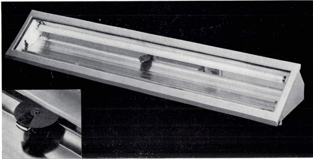
Fig. 17. The resistor combination R_2 (see fig. 14) is divided over several fluorescent lamp fittings. The light-transmission of the small rotatable discs varies with angle. The discs can be used to vary the amount of light received from the lamp by the light-sensitive resistors.
