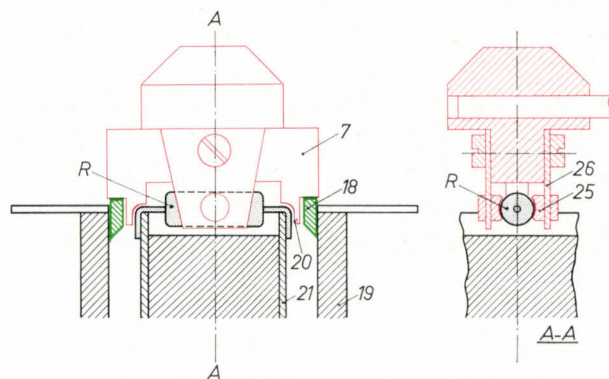
Fig. 4. Mechanism for cutting and bending the connection wires and for gripping the component. The head 7 (red) pushes the cutters 18 (green) down the inside surface of plates 19, thus cutting off the wires. Stud 20 then bend the wires around plates 21. The body of the component R is gripped by two nylon pads 25 which are pushed against the component by two springs 26.
