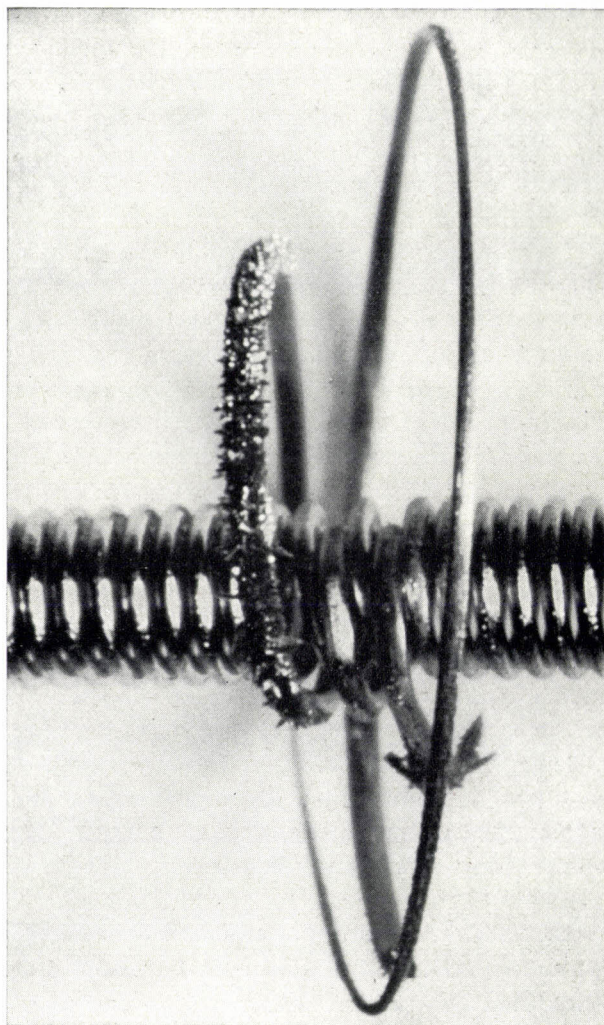
Fig. 2. Typical dendritic growth on the filament supports, due to surplus bromine. Magnification 20 \times .
