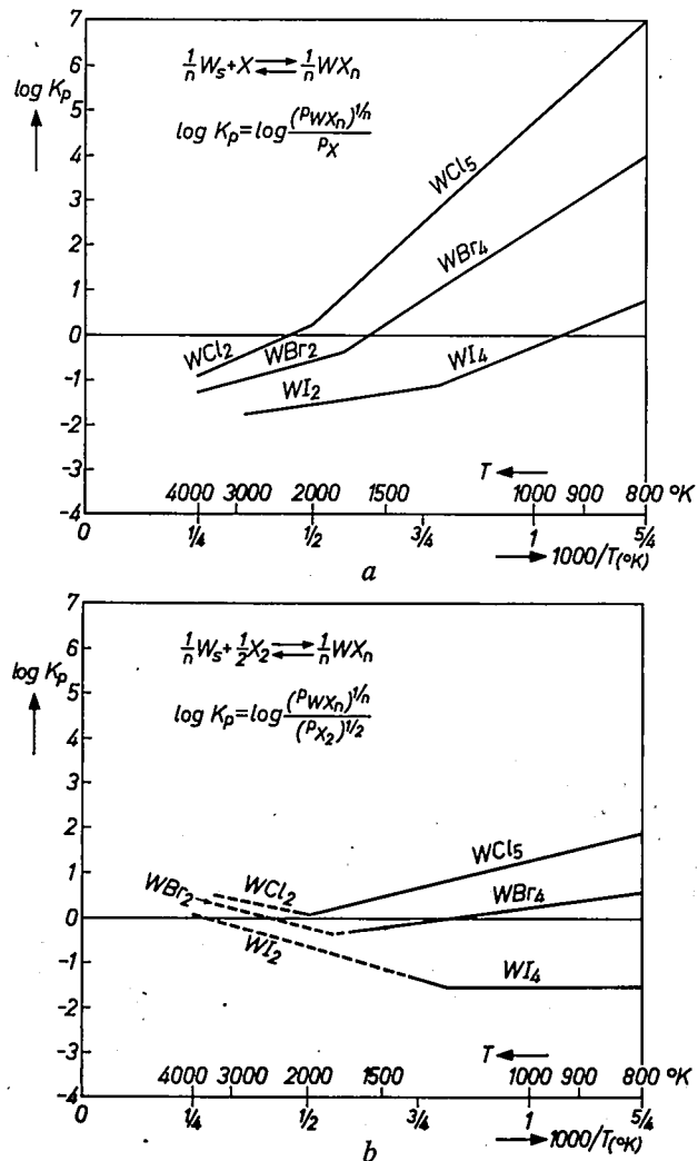
Fig. 1. A rough indication of the equilibrium constant K_p as a function of temperature T , for the reactions between solid tungsten and iodine, bromine or chlorine, in a) the atomic and b) the molecular state. The dashed part of the curves in (b) is only of theoretical significance, as in this temperature range the halogen can only exist in an almost entirely atomic state.
