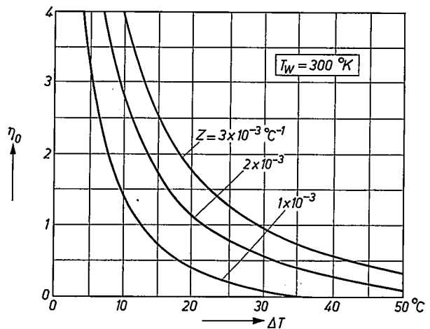
Fig. 13. Maximum efficiency \eta_0 as a function of the temperature reduction \Delta T for various values of the figure of merit Z . The hot junction temperature here is T_W = 300 \text{ }^\circ\text{K} .
