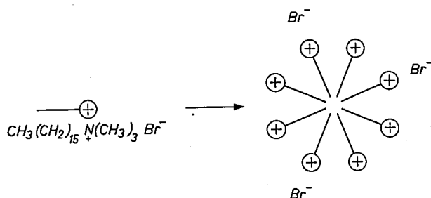
Fig. 10. Detergent or soap molecules have the tendency to unite into spherical micelles when above a certain concentration, the critical micelle concentration. A molecule of detergent consists of a non-polar part (thin line) and a polar part \oplus , each of which tries to find a similar medium. In the above sketch it is assumed that the solvent is polar, e.g. water.
