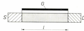
Fig. 3. Model of a thin-film transistor, used for the explanation of the characteristics. The letters and hatching have the same significance as in fig. 2. The length of the channel is l .
